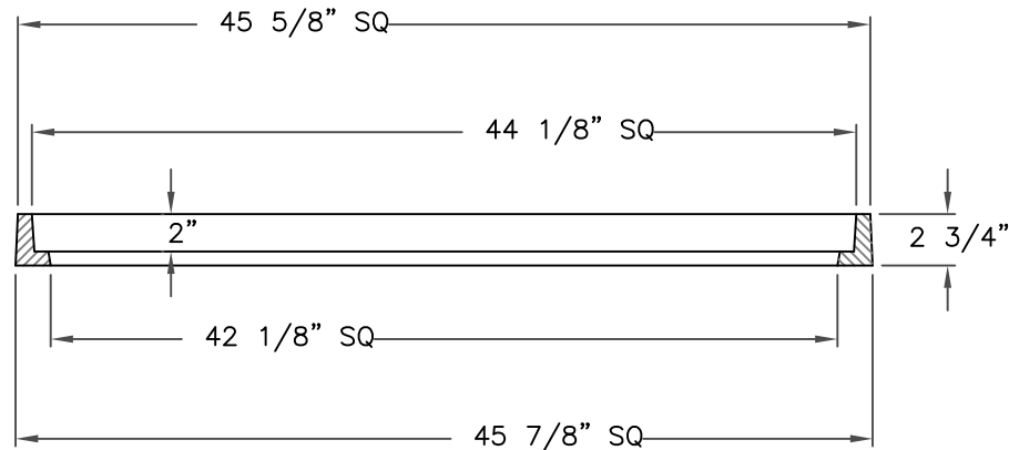
FRAME SECTION
